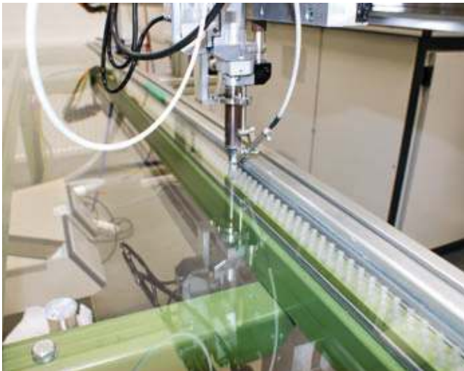
Ultrasonic soldering station
